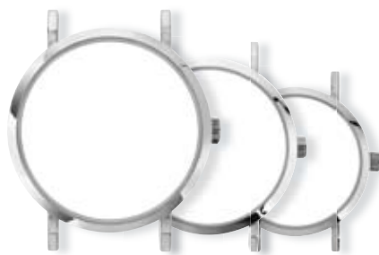
02 Gents: Case Size: ø40mm, Print size: ø34.5mm Unisex: Case Size: ø35mm, Print size: ø30mm Ladies: Case Size: ø30mm, Print size: ø25mm Finishing: Shiny / Matt
